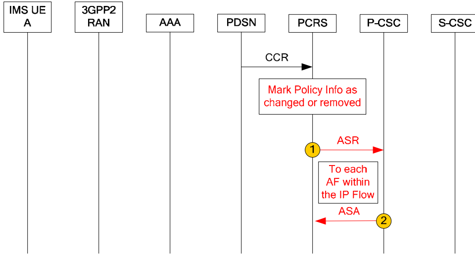
Figure 5: Example message flow that triggers AS-R/AS-A commands
